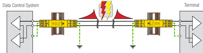
DIN-rail socket + pluggable SPD-module
